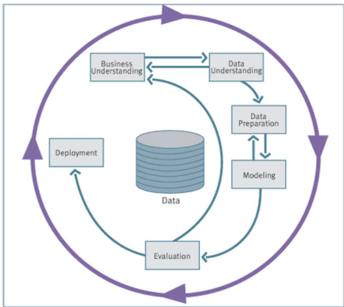
Figure 11: CRISP-DM Approach
